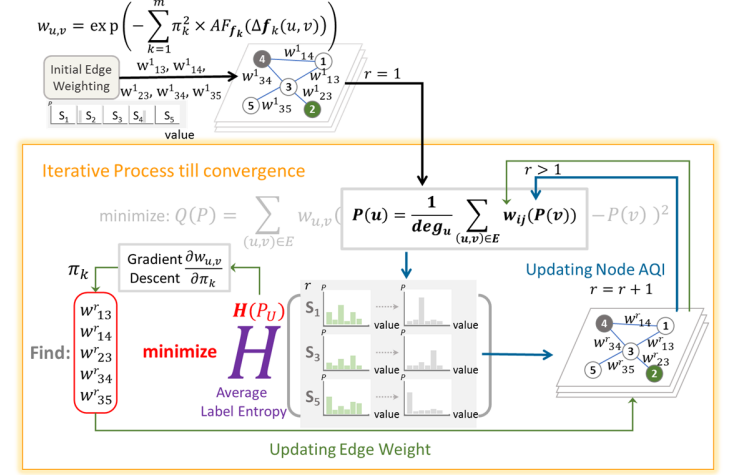
Figure 4. The process of inferring AQI values.
