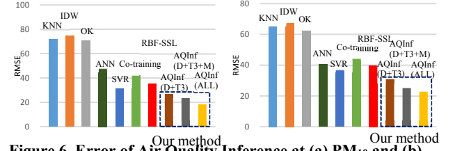
Figure 6. Error of Air Quality Inference at (a) PM_{10} and (b) PM_{2.5} for different algorithms.
