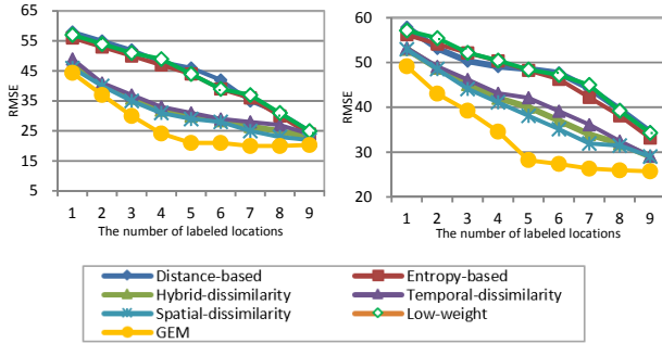
Figure 11. The RMSE of recommending 5 locations for PM 10 and PM 2.5 with varying number of labeled locations.
