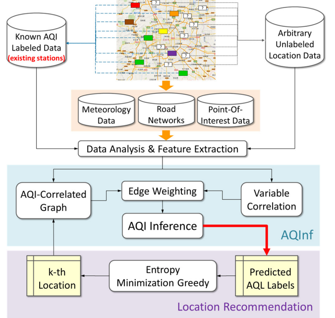
Figure 2. The proposed framework.
