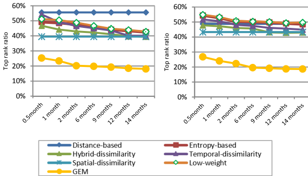
Figure 12. The TRR results for PM 10 and PM 2.5 when varying the length of time span N_T .
