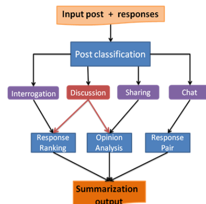
Figure 1. System architecture
